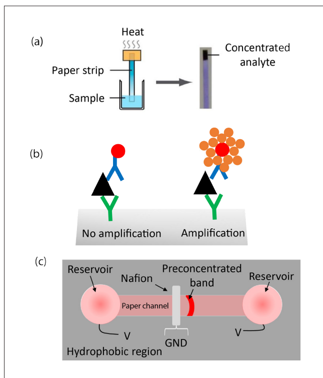
Figure 1. Three major signal amplification strategies in paper microfluidics. (a) The solvent evaporation method for analyte preconcentration. (Reprinted with permission from [3]; Copyright (2014) American Chemical Society). (b) A schematic of signal enhancement by nanoparticle catalyzed reduction in nanoparticle label assays. (c) Schematic of ion concentration polarization method of preconcentration.
